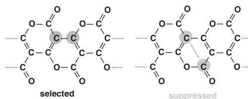
Figure 3. ^{13}\text{C} - ^{13}\text{C} spin pairs selected and suppressed by ^{13}\text{C} double-quantum double-filtering NMR; the underlying grey circles mark ^{13}\text{C} nuclei; only spin pairs connected over a CC bond contribute to the double-quantum filtered signal; the spin pair shown on the right-hand side has negligible J coupling and is filtered out.
