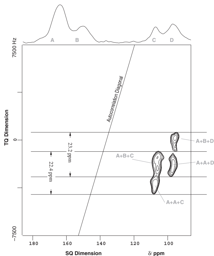
Figure 7. 2D triple-quantum filtered correlation spectrum of poly(carbonsuboxide) (sample I) using the through-bond dipolar coupling for triple-quantum coherence excitation (pulse sequence c, Figure 2).
