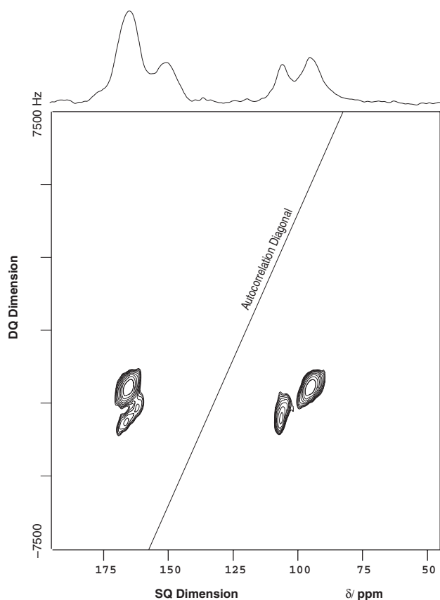
Figure 6. 2D double-quantum filtered correlation spectrum of poly(carbonsuboxide) (sample II) using the through-bond dipolar coupling for double-quantum coherence excitation (pulse sequence a, Figure 2).
