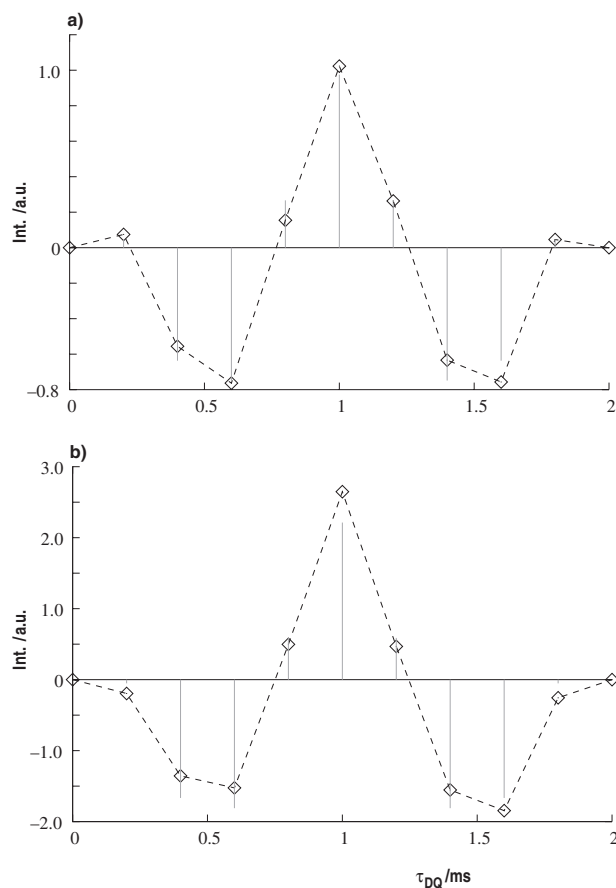
Figure 9. Double-quantum constant-time double-filtering build-up curves for the resonances at 107.5 ppm (lower curved labeled B) and 96 ppm (upper curve marked a) of poly(carbonsuboxide) (sample II), acquired at \nu_r = 10 kHz spinning-speed (pulse sequence d, Figure 2); if no double-filtering is applied no zero-crossings can be observed in double-quantum constant-time build-up curves. \diamond : experimental, — (light grey): simulated.
