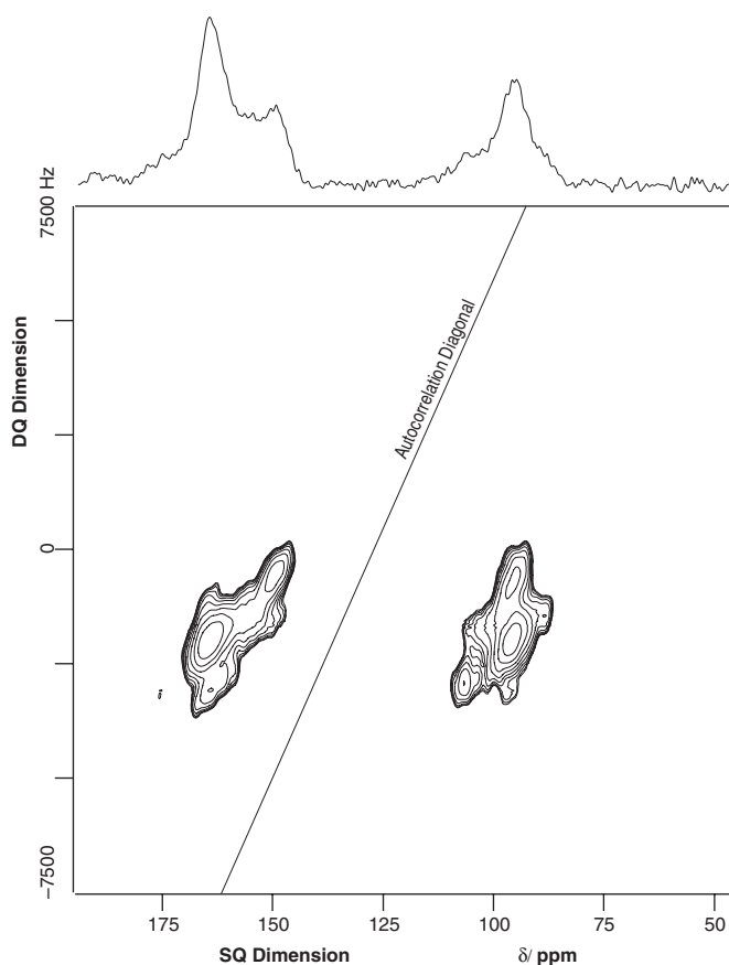
Figure 5. 2D double-quantum filtered correlation spectrum of polycarbonsuboxide (sample I) using the through-space dipolar coupling; the double-quantum/zero-quantum conversion times \tau_{\text{DQ}} with 1.067 ms are short enough to ensure that the double-quantum peak intensities reflect directly bound pairs.
