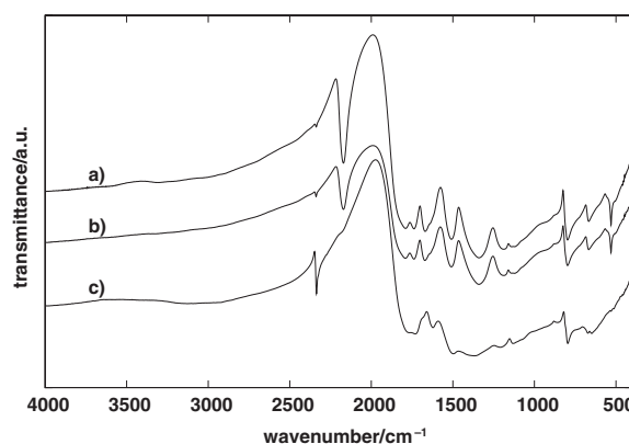
Figure 1. IR spectra of poly(carbonsuboxide); isotopes are at natural abundance; spectrum a refers to a sample which has not been exposed to air, spectrum b and c to a sample from the same charge which have been exposed to air for 2 and 5 s, respectively.
