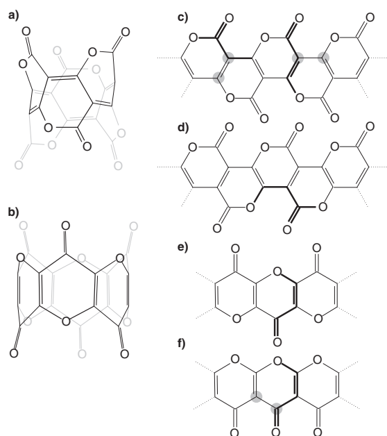
Figure 11. Model structures for poly(carbonsuboxide); marked in bold type are atoms belonging to the same monomer (structures c to f); the carbon atoms highlighted by grey circles refer to carbon atoms in an intermonomeric C_{CCC}-C_{CCO} bond.
