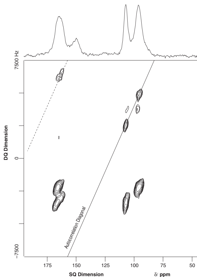
Figure 8. 2D double-quantum filtered correlation spectrum of poly(carbonsuboxide) (sample II) using the through-space dipolar coupling; the autocorrelation signal at 163 ppm is folded over the edge; the fold-over autocorrelation diagonal is indicated by a dashed line.
